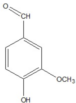
4-hydroxy-3-methoxybenzaldehyde
